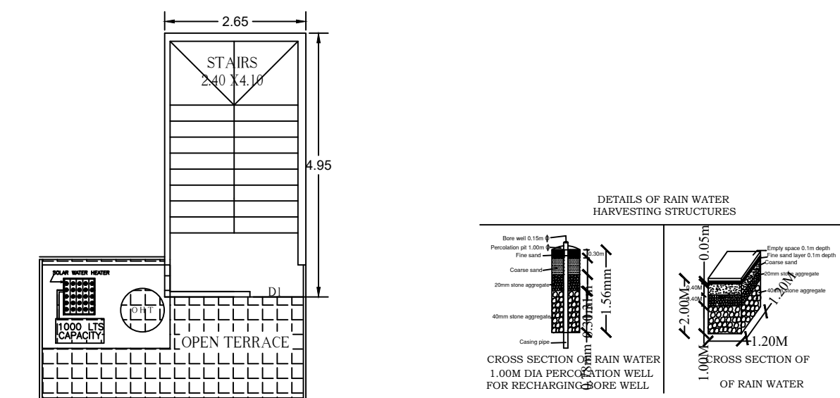
TERRACE FLOOR PLAN
