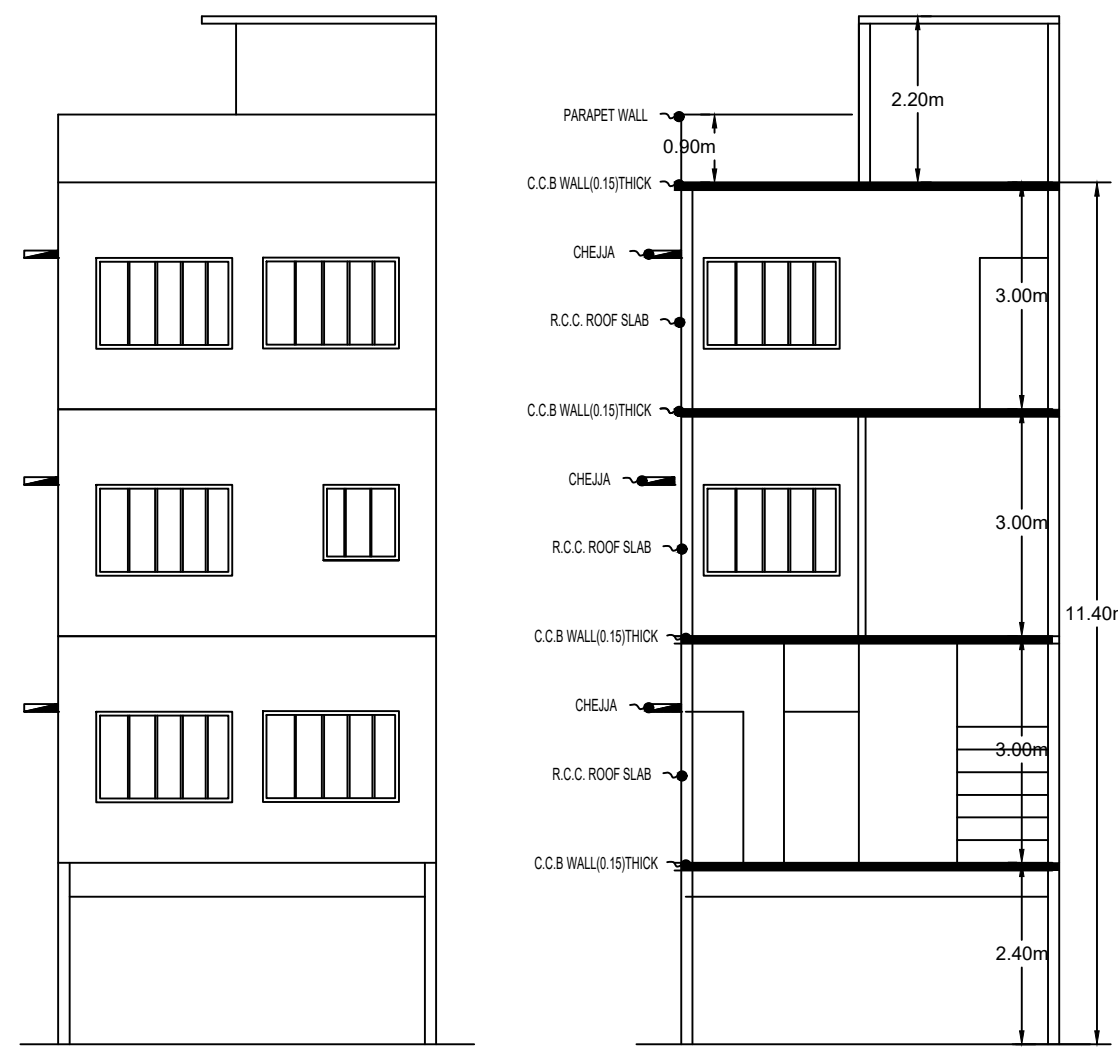
SECTION @ X-X'
